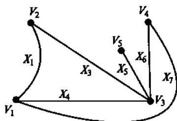
G = G_1 \cup G_2
