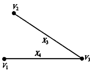
G' = G_1 \cap G_2
